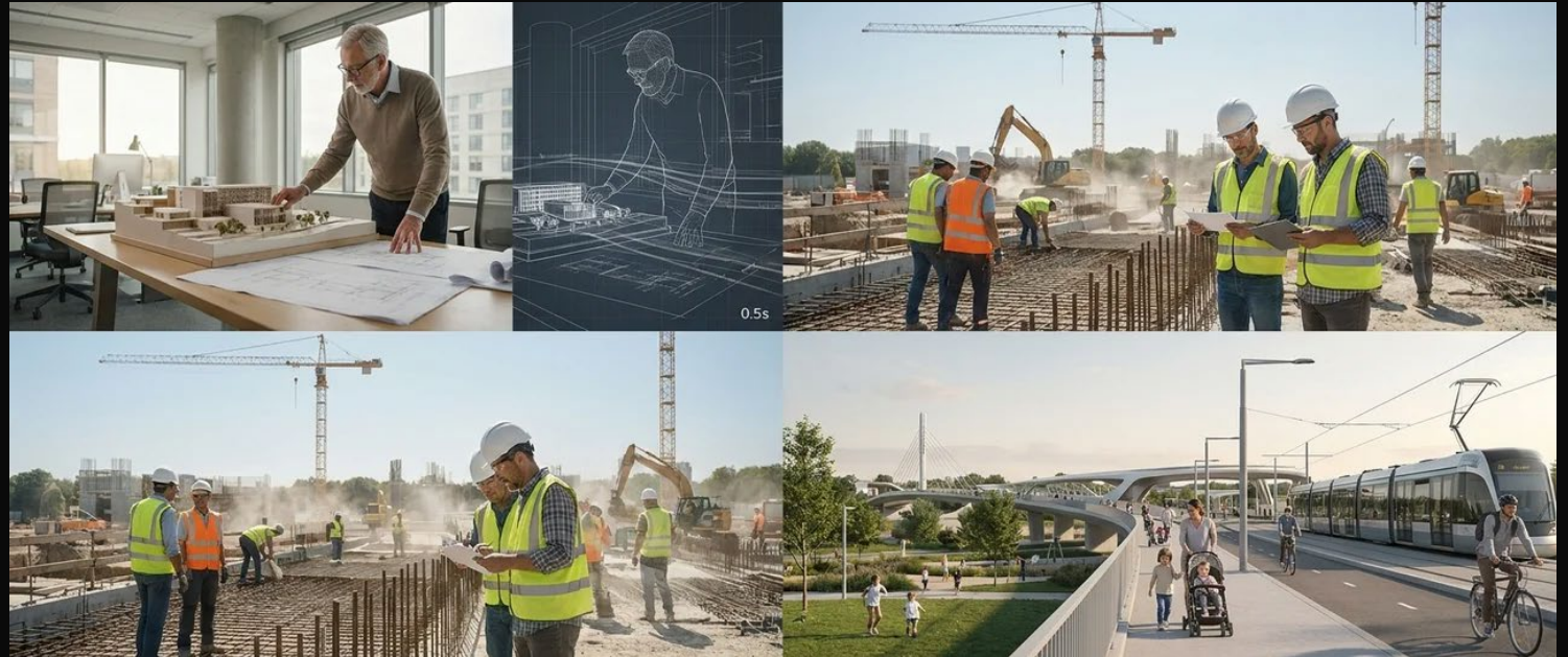
Concept Exploration
